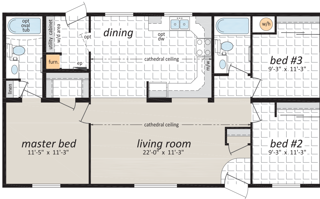
"The AM-861" 24' x 44' 1,056 sq.ft.
