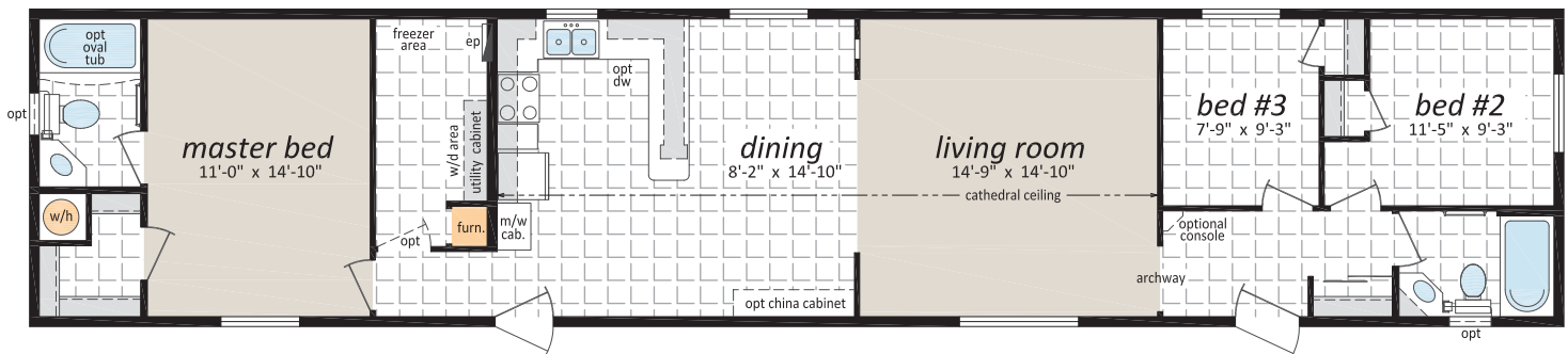
“The AM-877” 16' x 76' 1,216 sq.ft.
