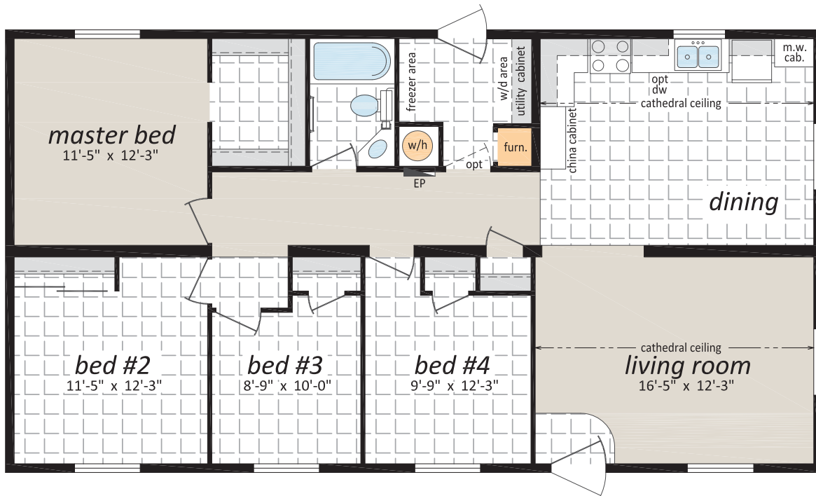
"The AM-858" 26' x 48' 1,248 sq.ft.
