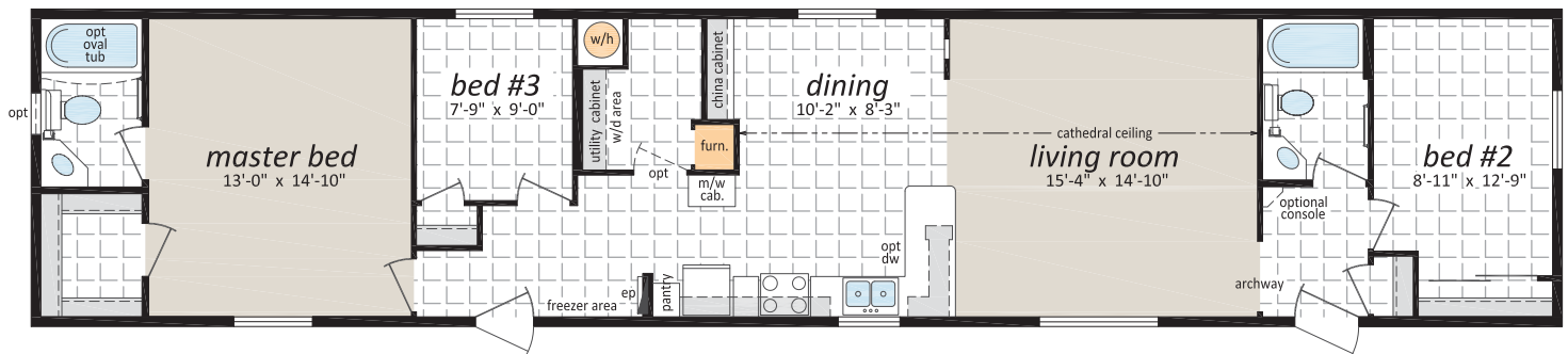
"The AM-816" 16' x 76' 1,216 sq.ft.
