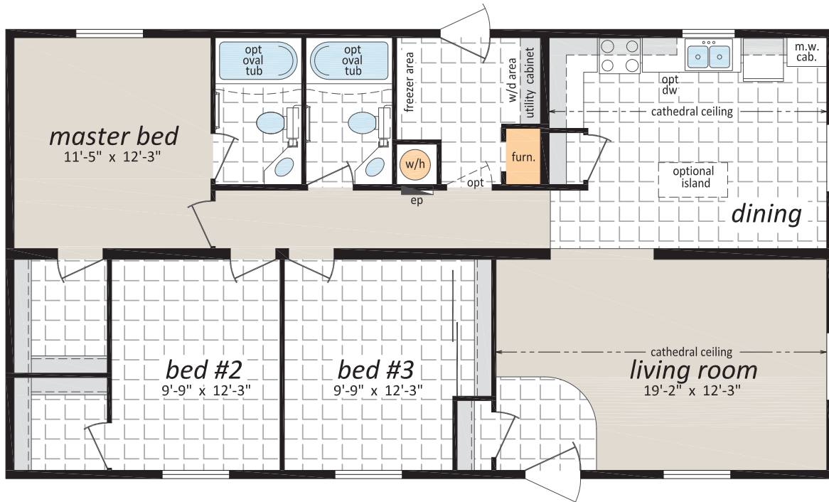
"The AM-860" 26' x 48' 1,248 sq.ft.
