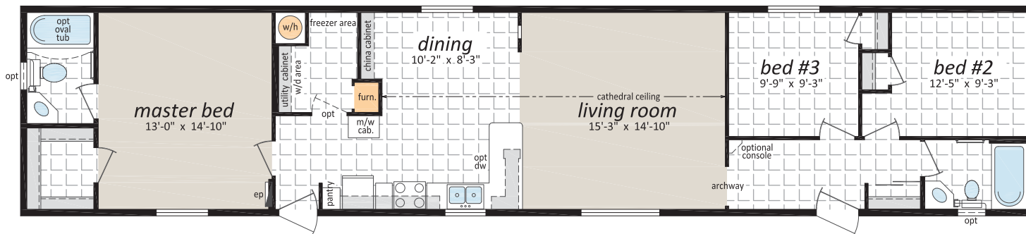
“The AM-810” 16' x 76' 1,216 sq.ft.
