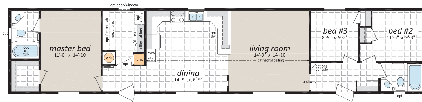
“The AM-898” 16' x 76' 1,216 sq.ft.
