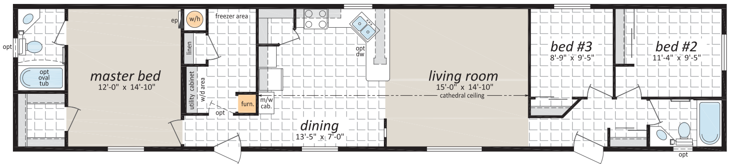
“The AM-886” 16' x 76' 1,216 sq.ft.
